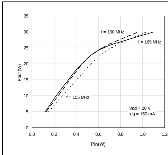
Figure 1. P_{OUT} vs P_{in} and frequency @ V_{dd} = 20\text{ V}
