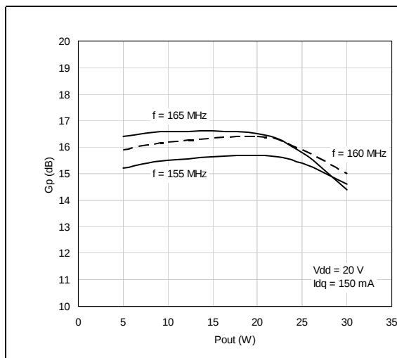
Figure 3. Gain vs P_{OUT} and frequency @ V_{dd} = 20\text{ V}
