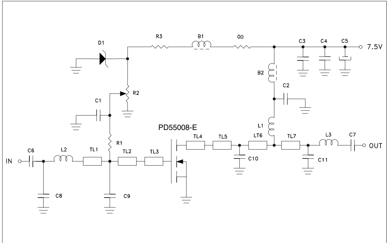
Figure 10. Circuit layout
