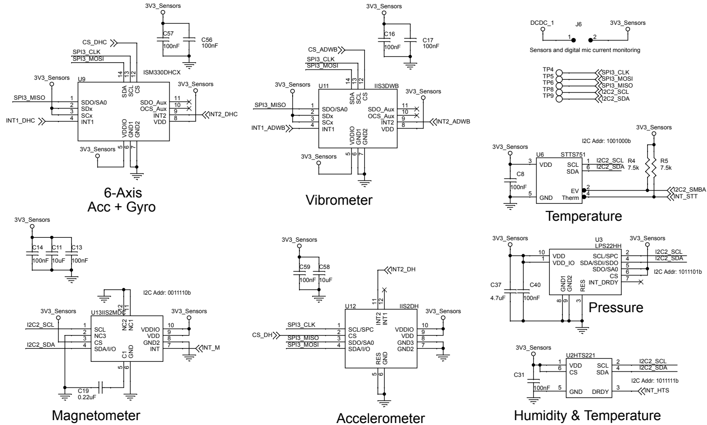
Figure 4. STEVAL-STWINKT1B schematic (3 of 7)
