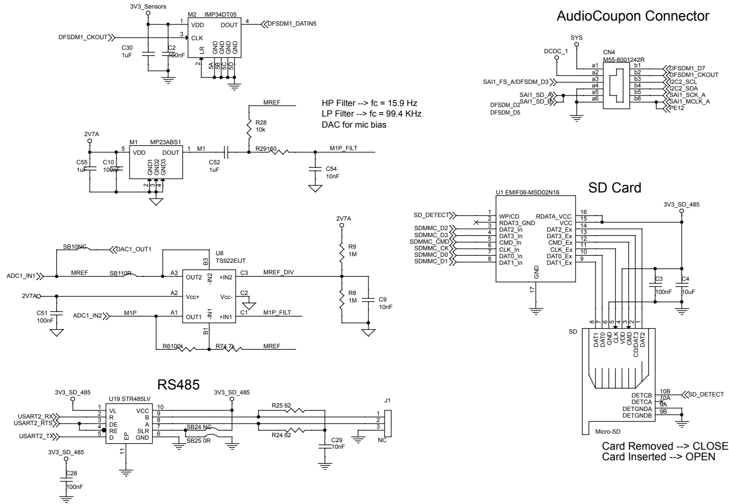
Figure 6. STEVAL-STWINKT1B schematic (5 of 7)
