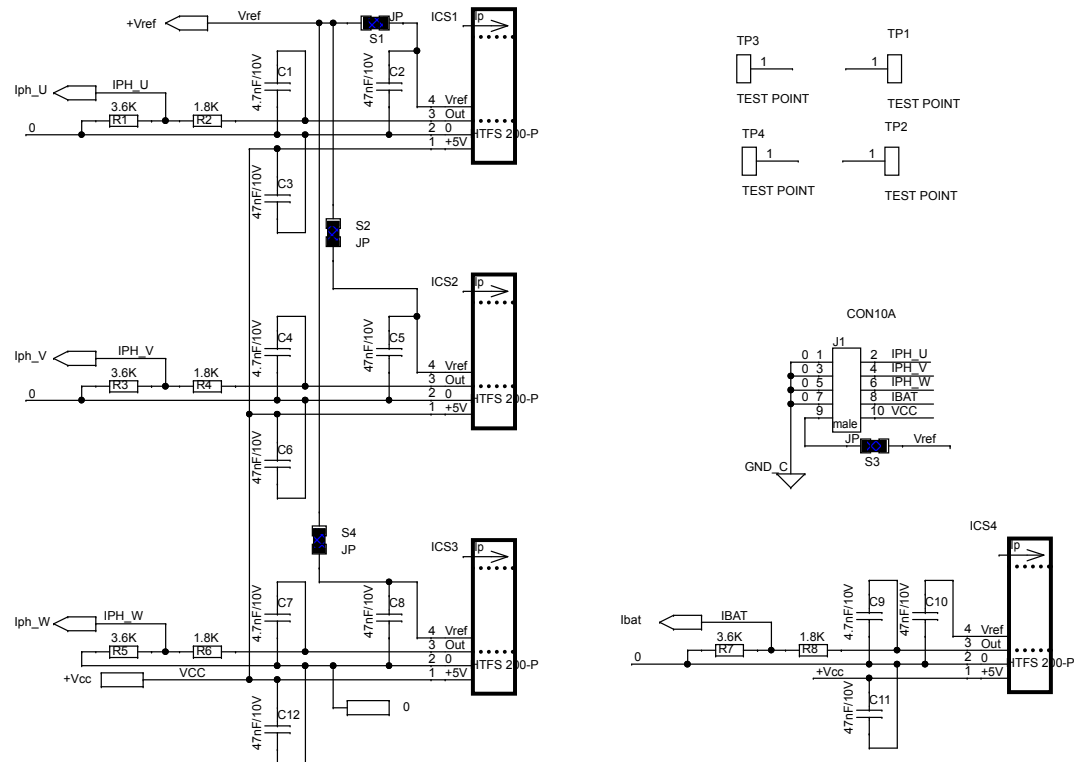
Figure 9. Current sensor board schematics
