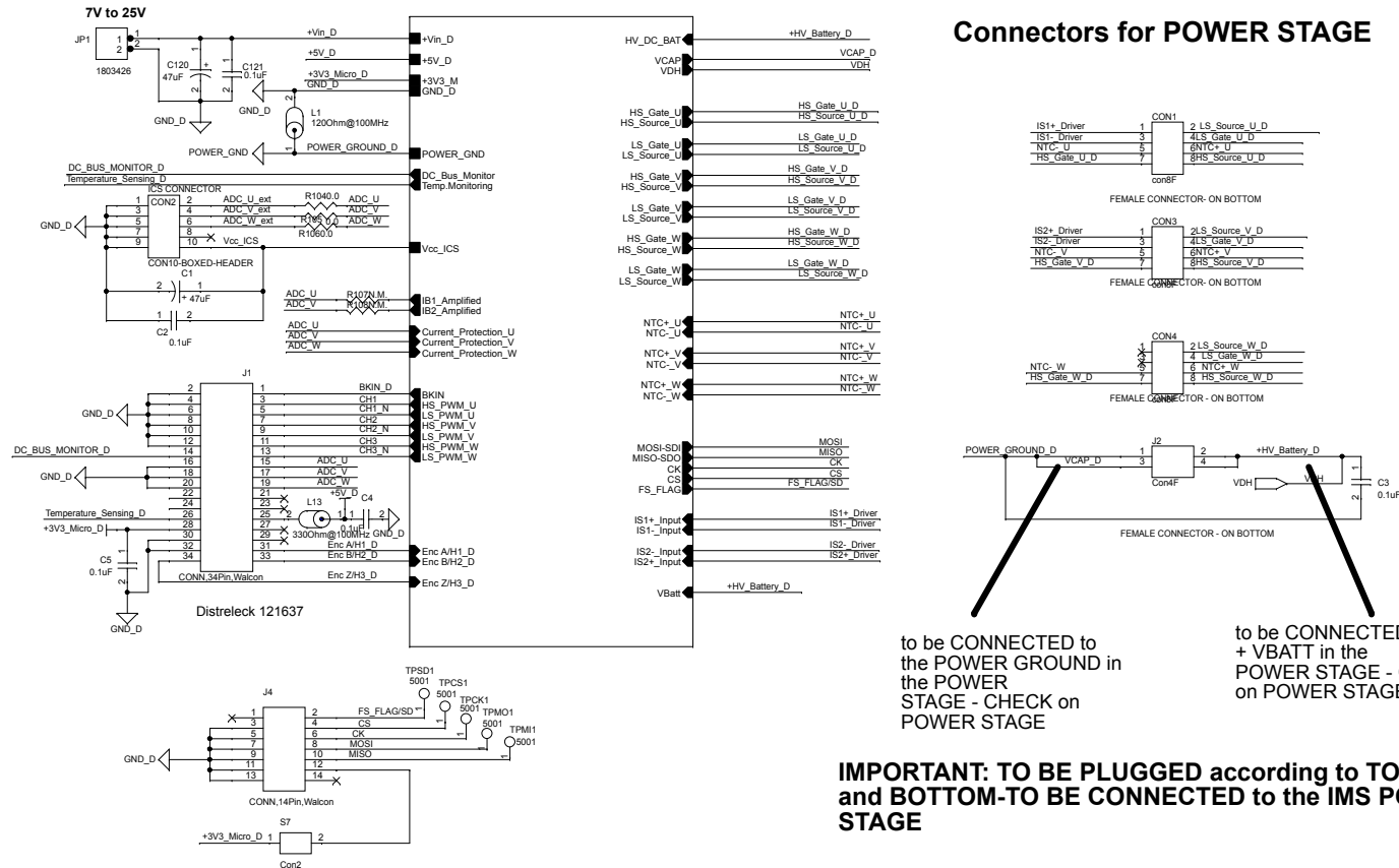
Figure 4. Driver board schematics - main with connectors
