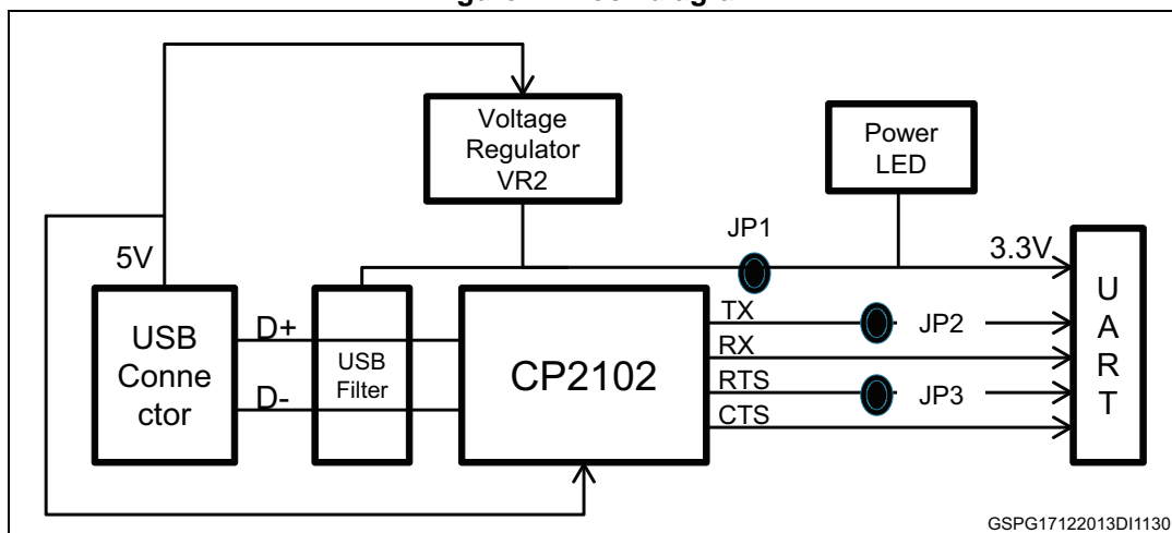
Figure 2. Block diagram
