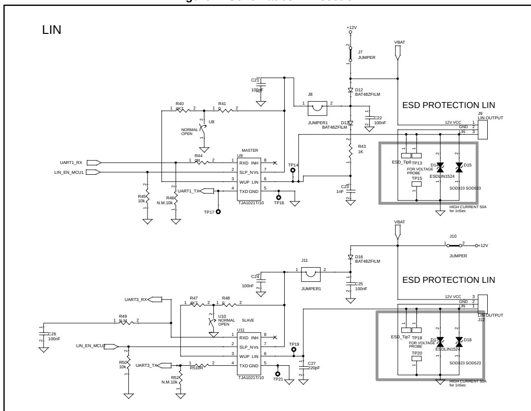
Figure 2: Schematics LIN section
