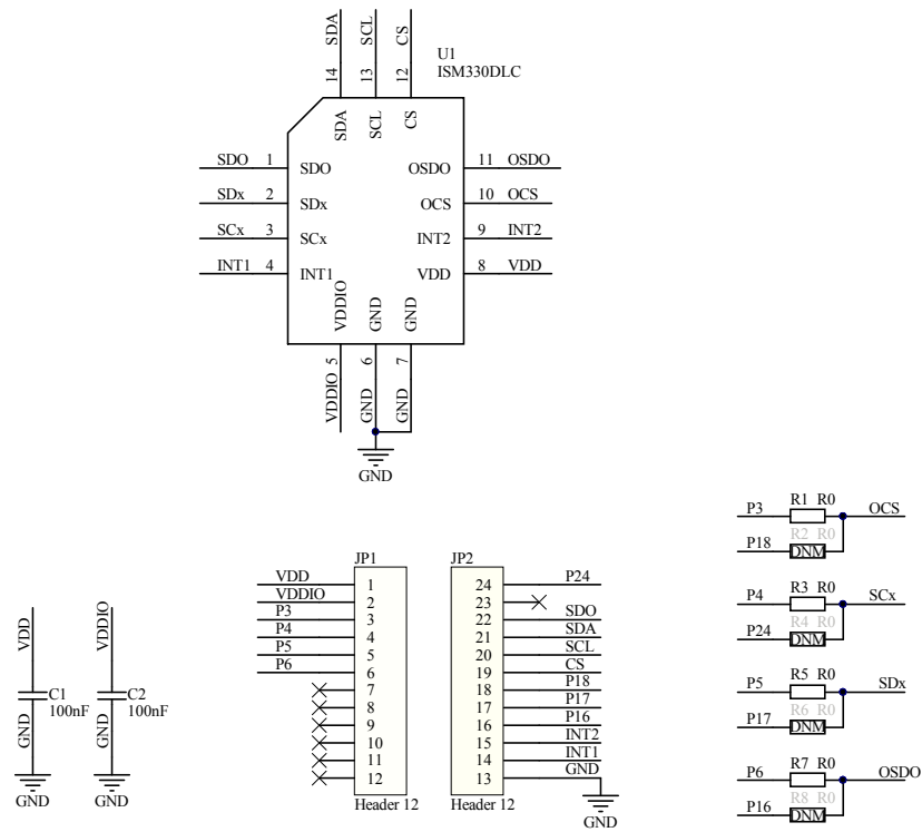
Figure 1. STEVAL-MKI182V2 circuits
