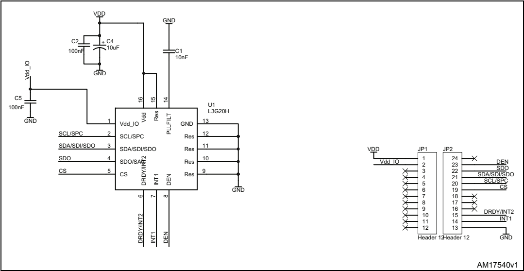
Figure 1. STEVAL- MKI136V1 circuit schematic
