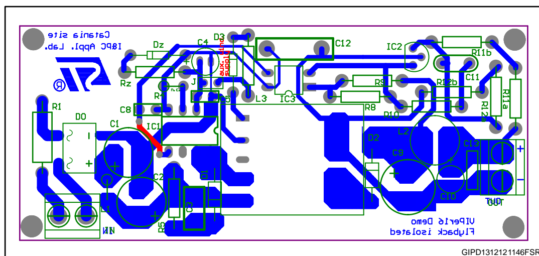
Figure 2: Board layout
