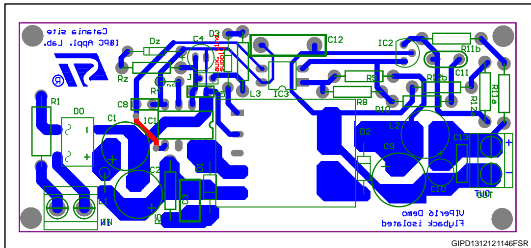
Figure 2: Board layout
