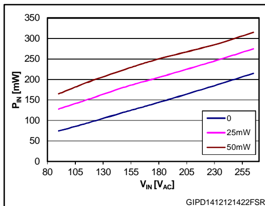
Figure 8: Standby consumption at no/light load: IC self biased (J not selected)
