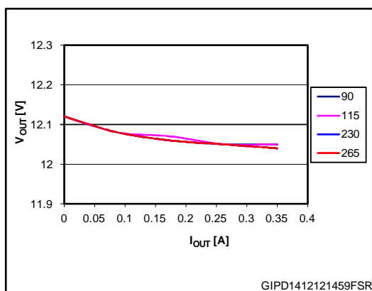
Figure 10: Load regulation
