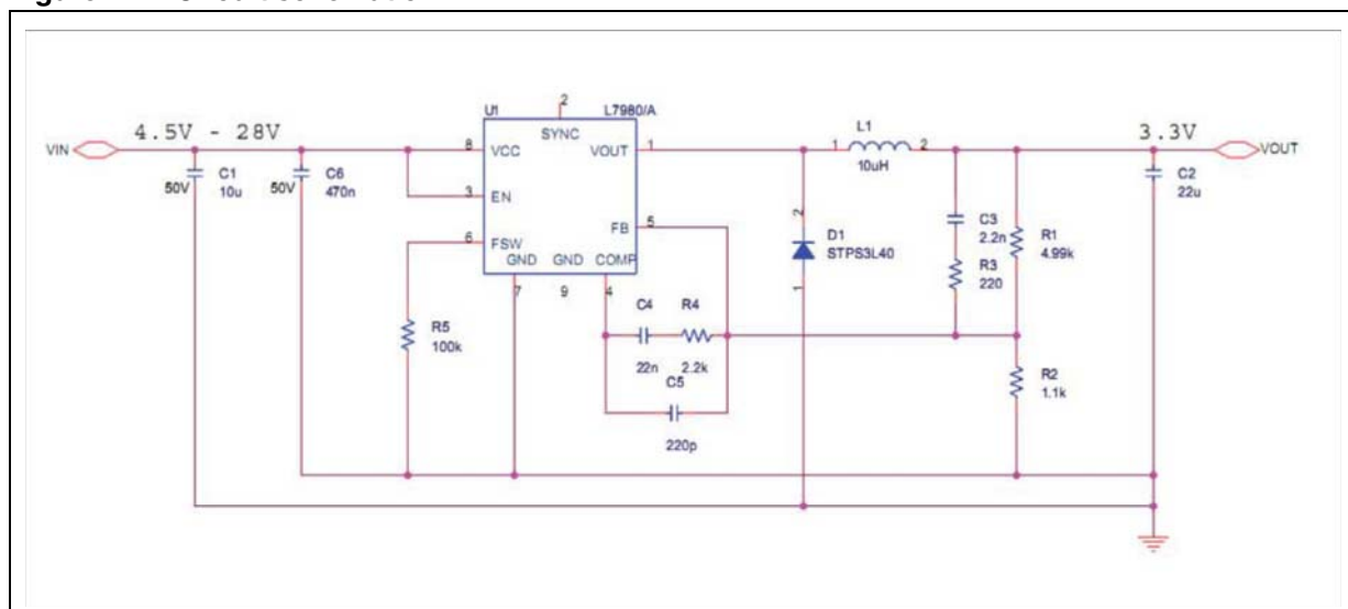
Figure 1. Circuit schematic
