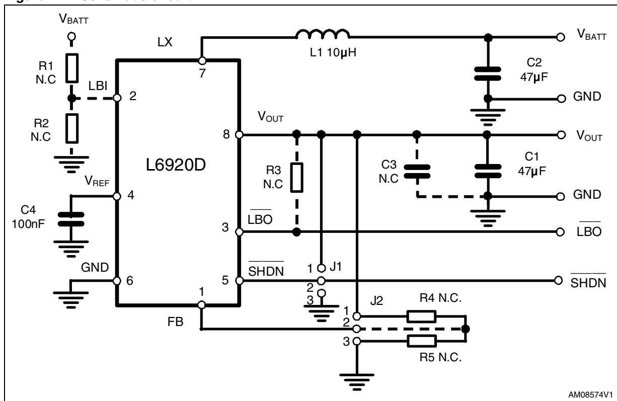
Figure 1. Schematic circuit
