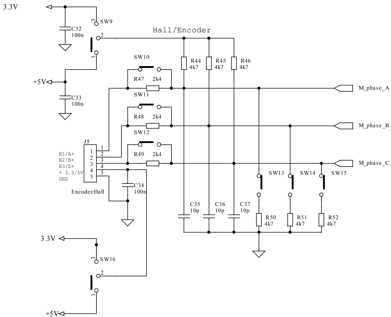
Figure 5. STEVAL-IPM20B board schematic (5 of 5)
