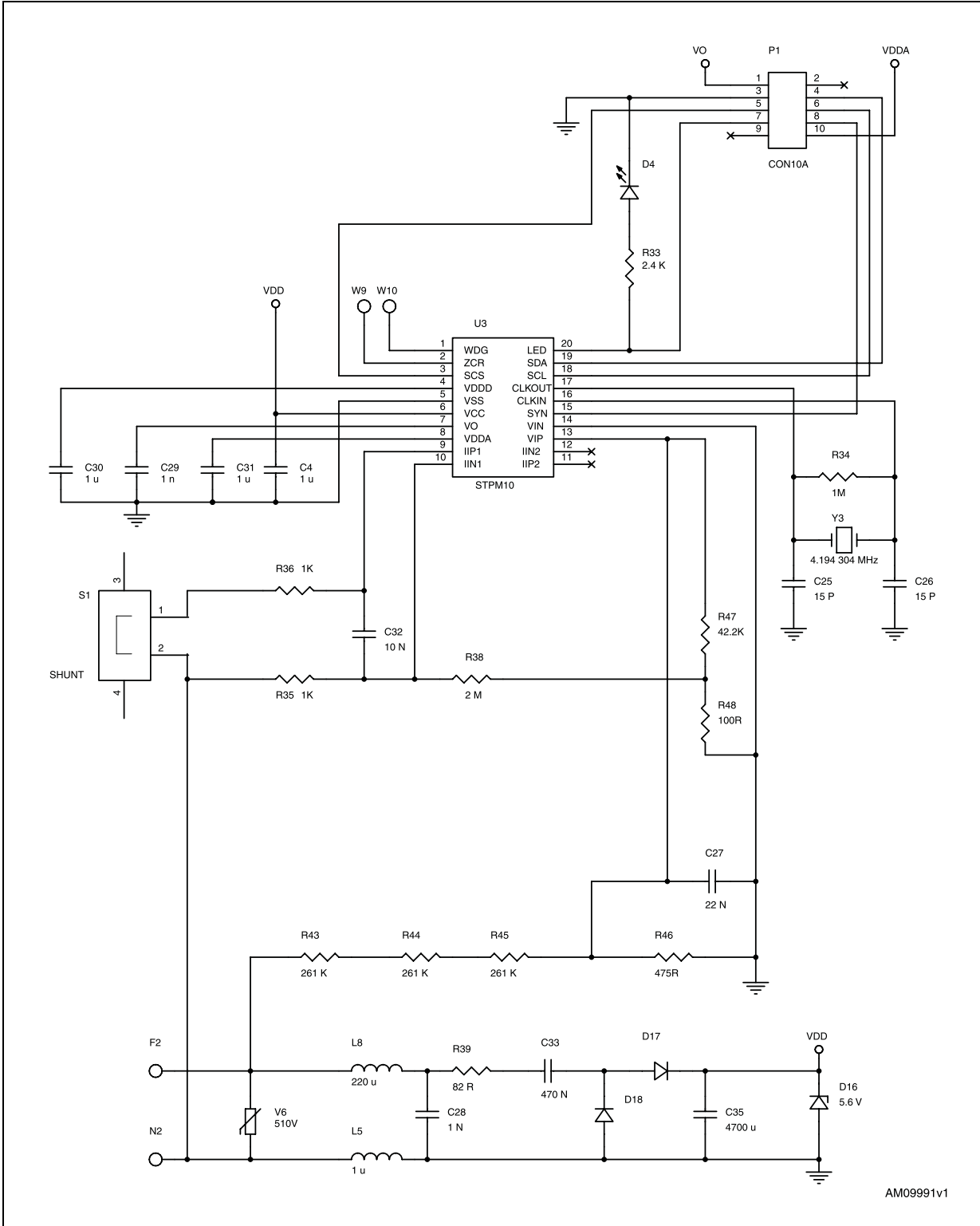
Figure 1. Schematic circuit
