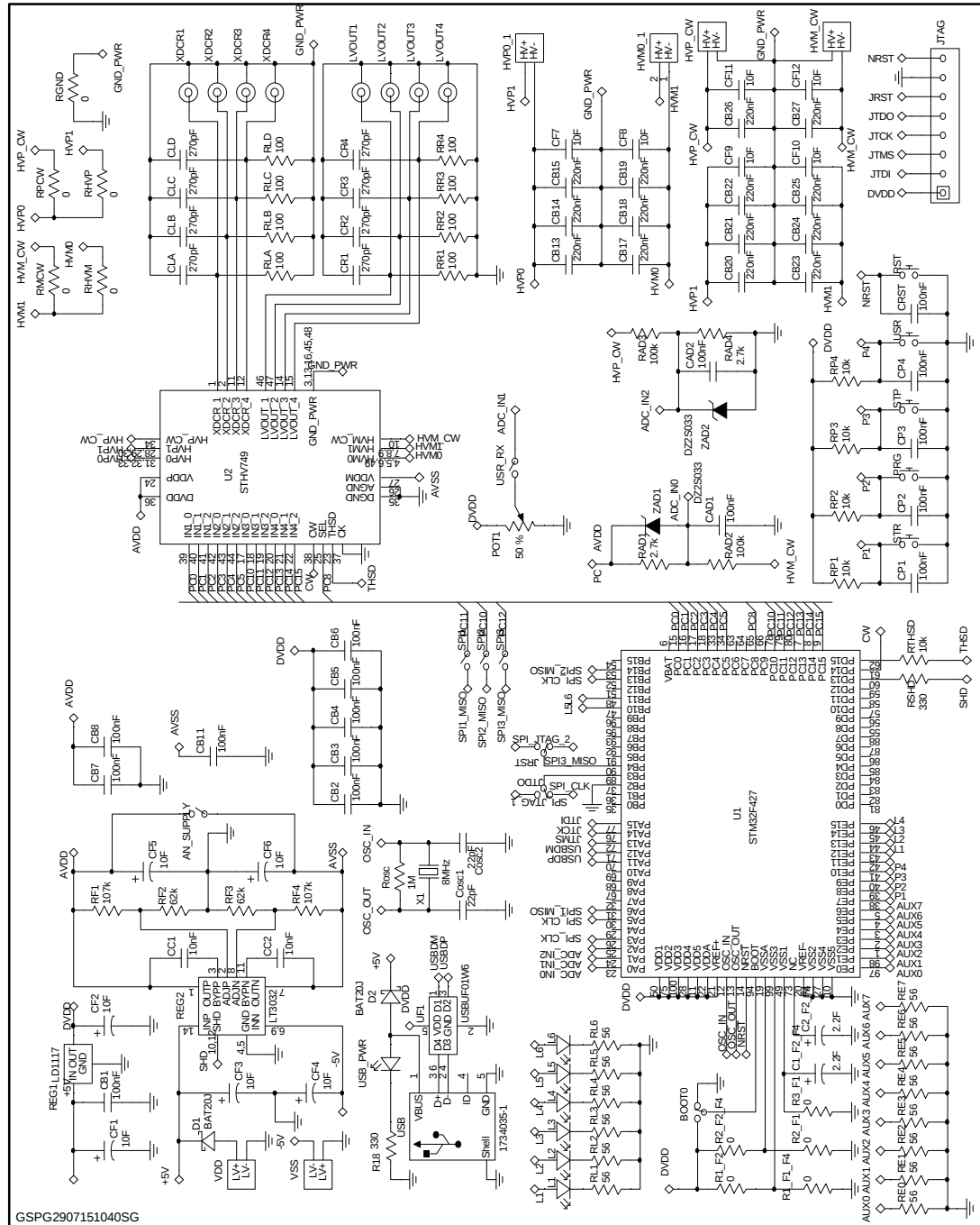
Figure 1: STEVAL-IME012V1 circuit schematic
