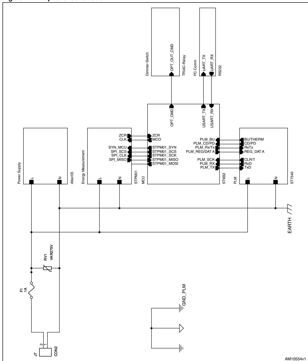
Figure 1. Top-level schematic
