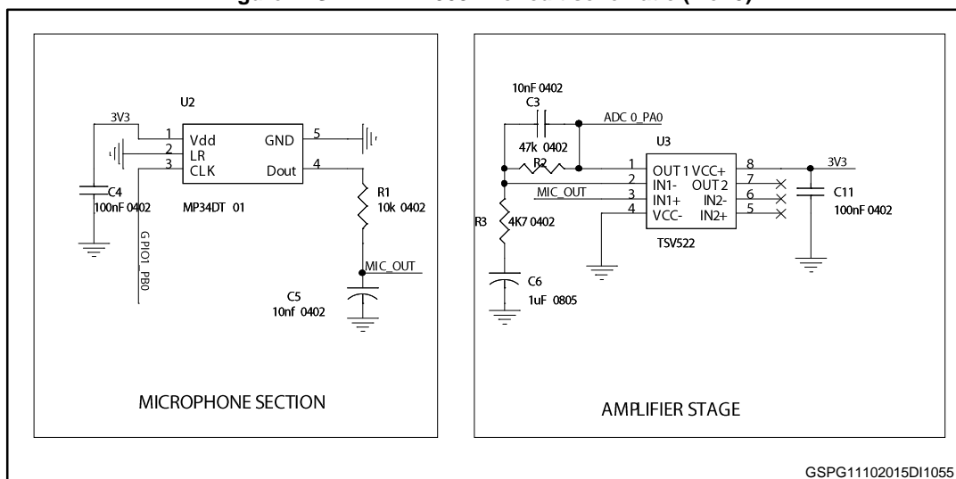
Figure 2: STEVAL-IDI003V2 circuit schematic (2 of 5)
