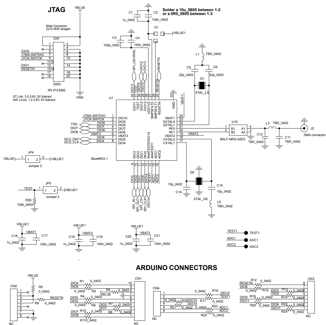
Figure 1. STEVAL-IDB007V2 - scheme 1
