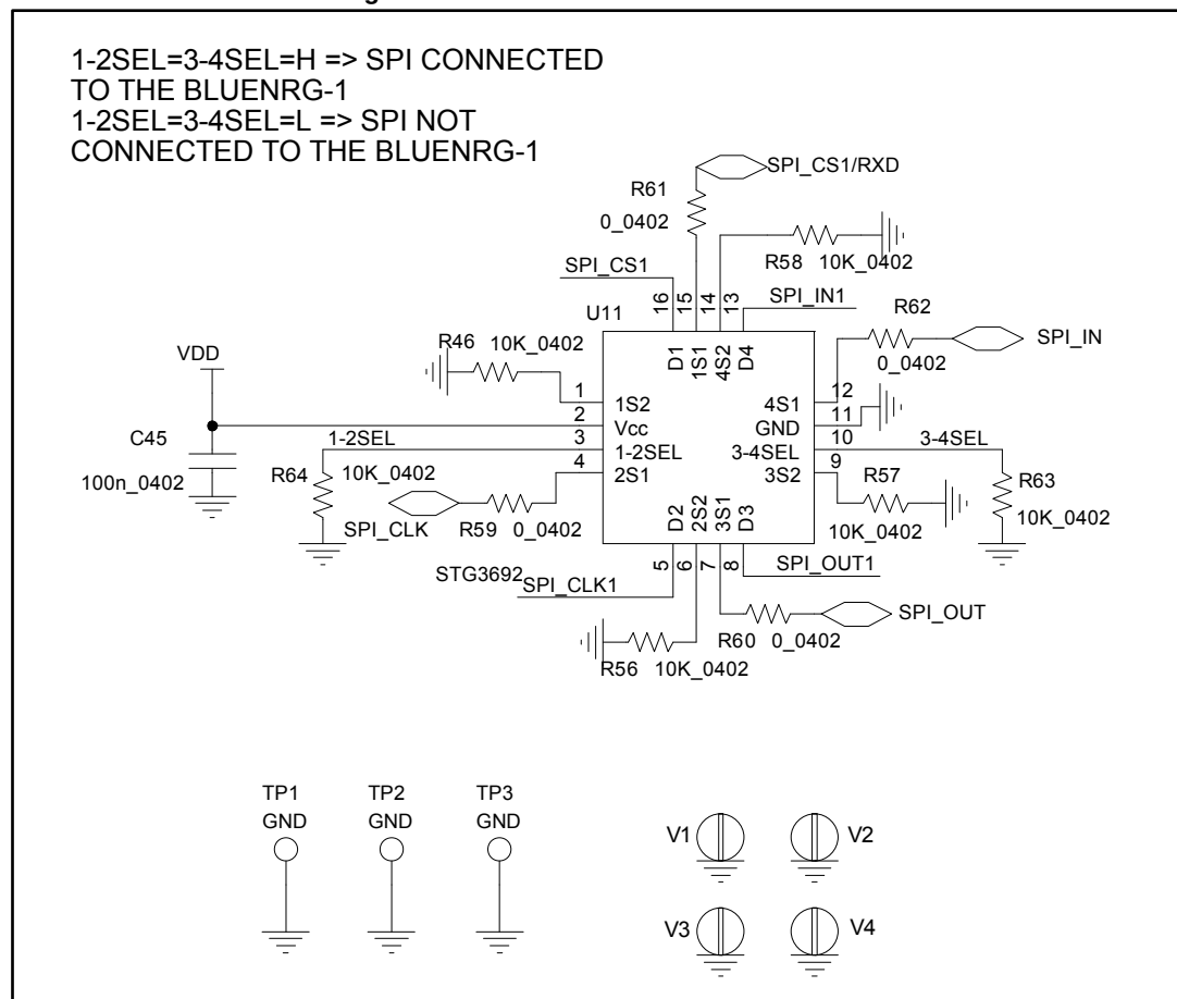
Figure 8: STEVAL-IDB007V1M - EEPROM
