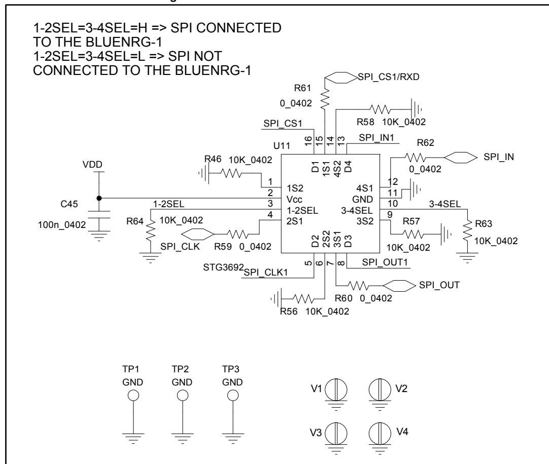
Figure 8: STEVAL-IDB007V1M - EEPROM
