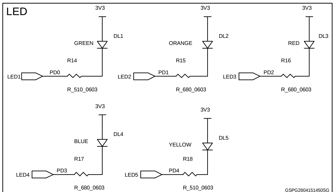
Figure 7: LED
