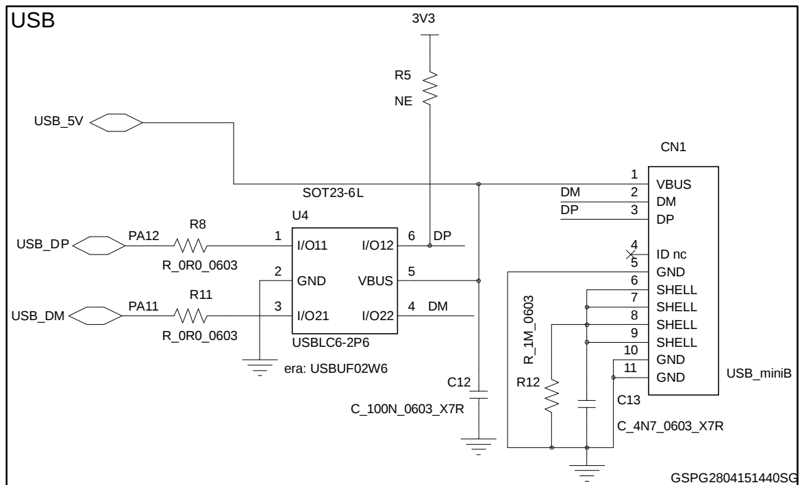
Figure 6: USB
