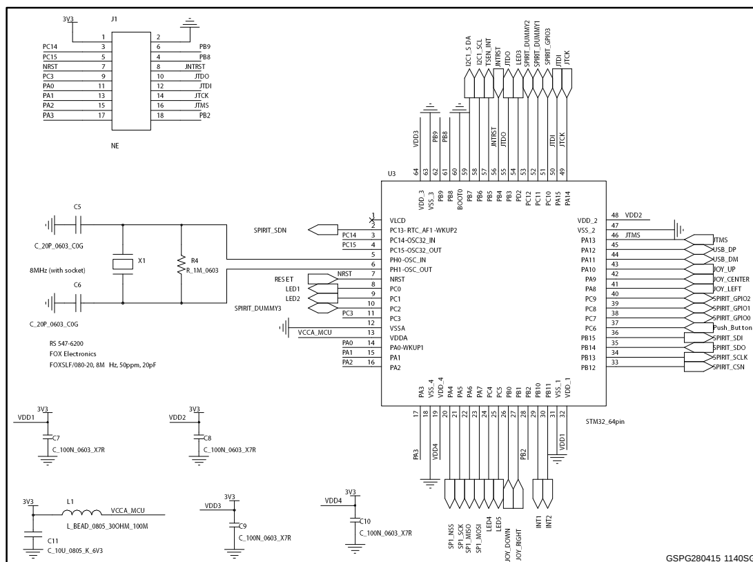
Figure 4: MCU
