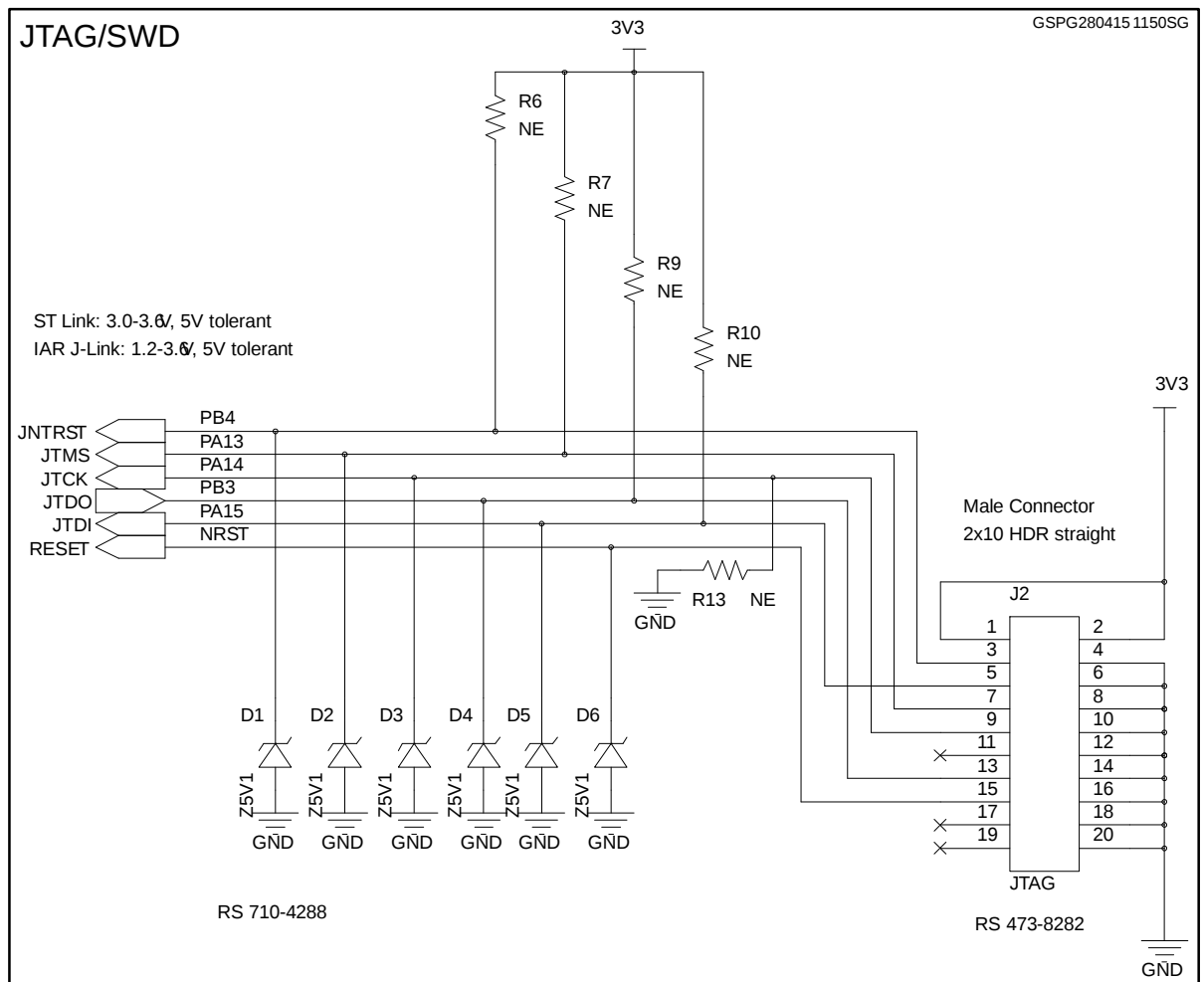
Figure 5: JTAG / SWD
