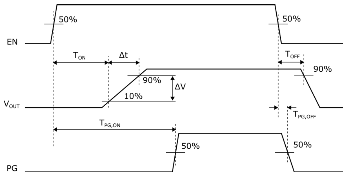
Figure 5. Switching characteristics timing
