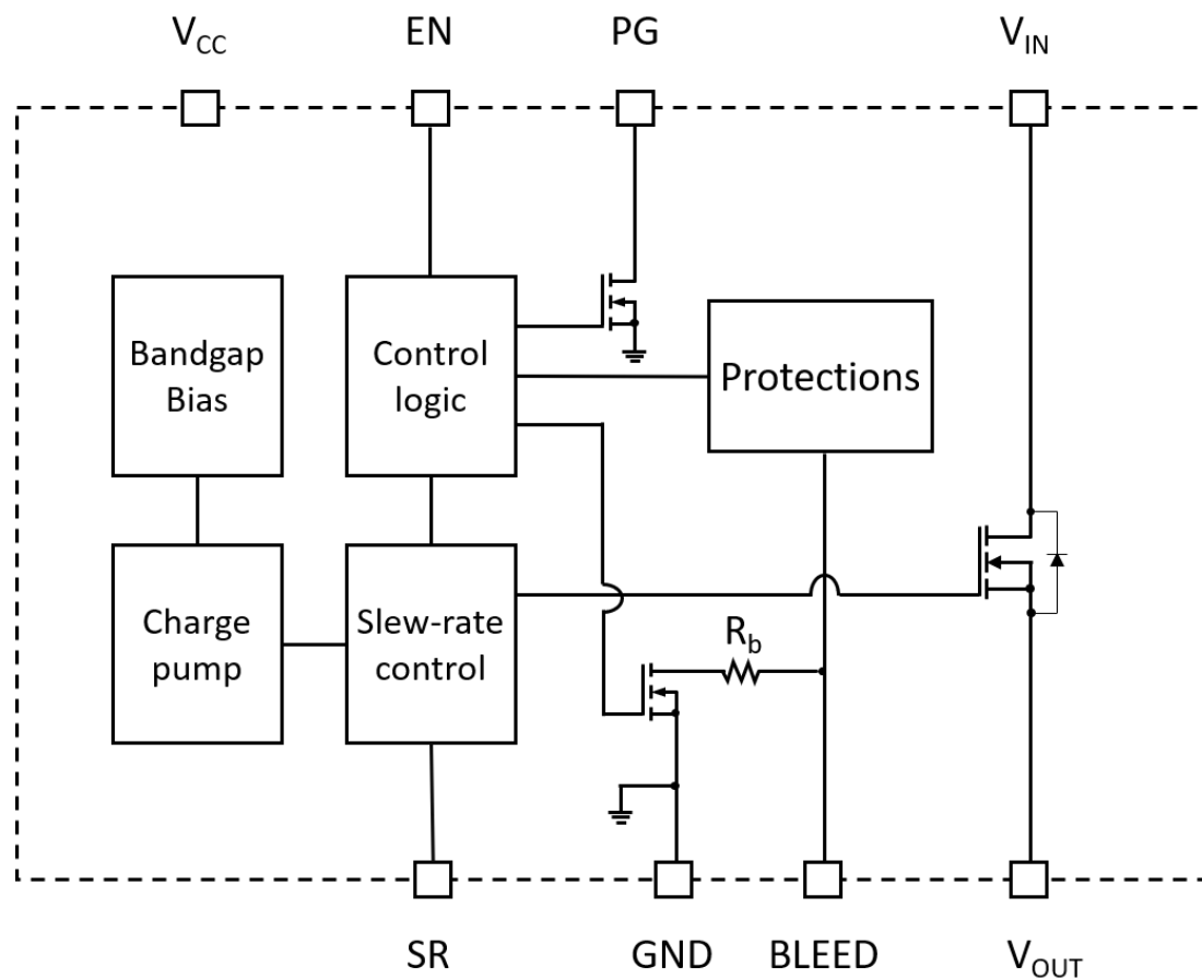
Figure 1. Block diagram
