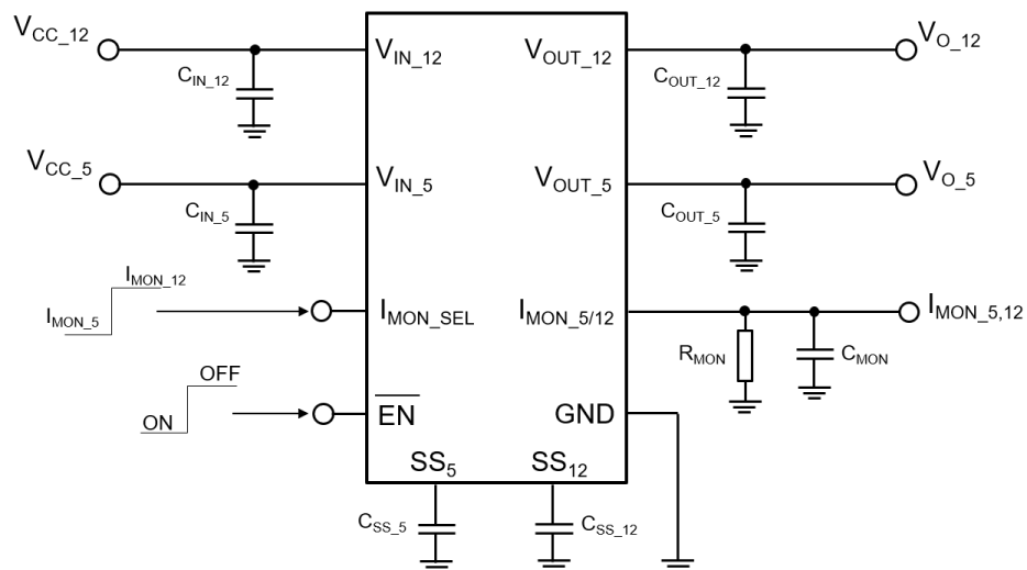
Figure 3. Typical application circuit
