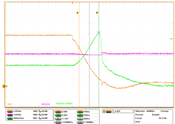
Figure 40. PLP protection through UVLO_5
