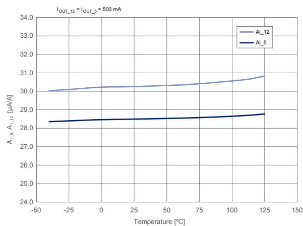
Figure 22. Current monitor gain vs. temperature
