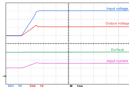
Figure 20. Voltage clamp
