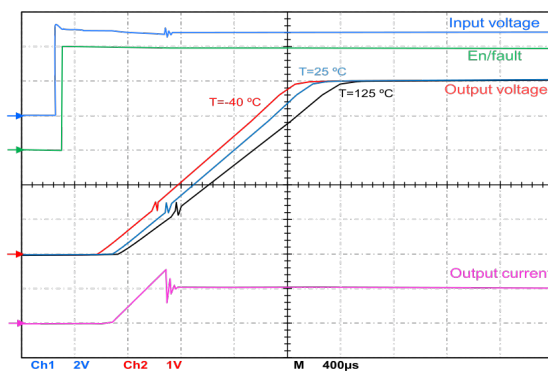
Figure 13. V_{OUT} ramp-up vs enable (NO C_{dvd} )
