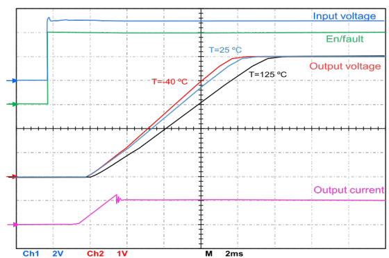
Figure 14. V_{OUT} ramp-up vs enable ( C_{dvd} = 470\text{ pF} )
