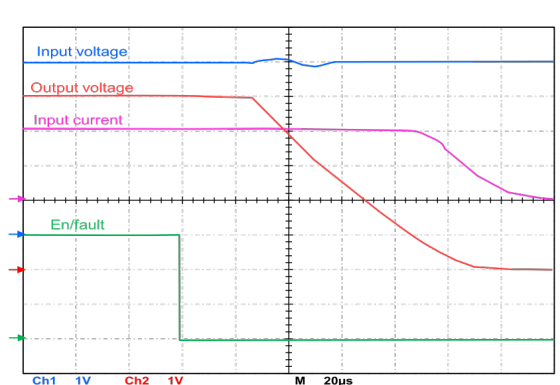
Figure 16. V_{OUT} turn-off vs enable
