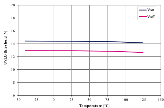
Figure 13. UVLO voltage vs. temperature
