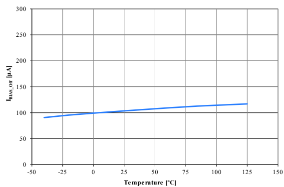
Figure 15. Off-state current vs. temperature
