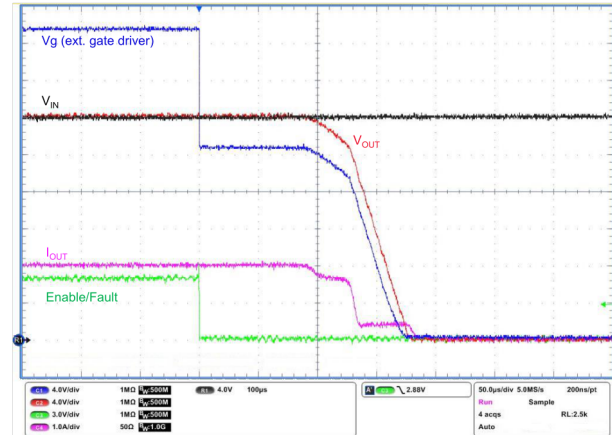
Figure 33. Enable turn-off with external FET
