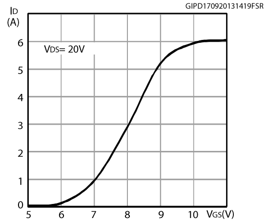
Figure 9: Transfer characteristics
