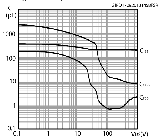
Figure 12: Capacitance variations
