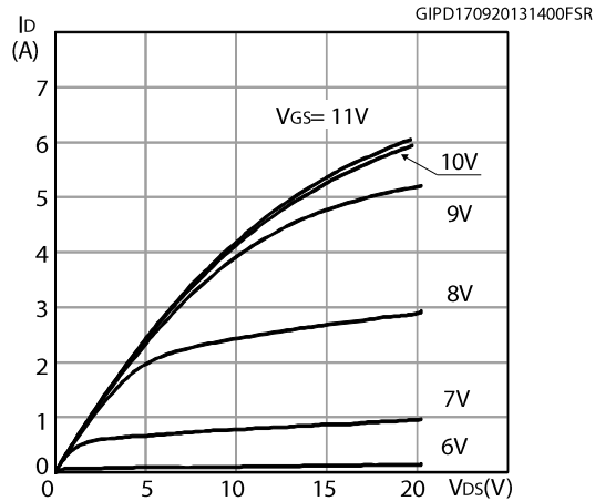
Figure 8: Output characteristics
