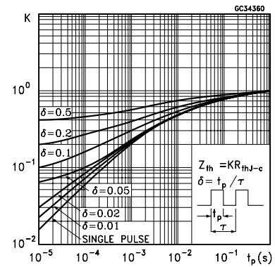
Figure 2. Thermal impedance for DPAK and IPAK
