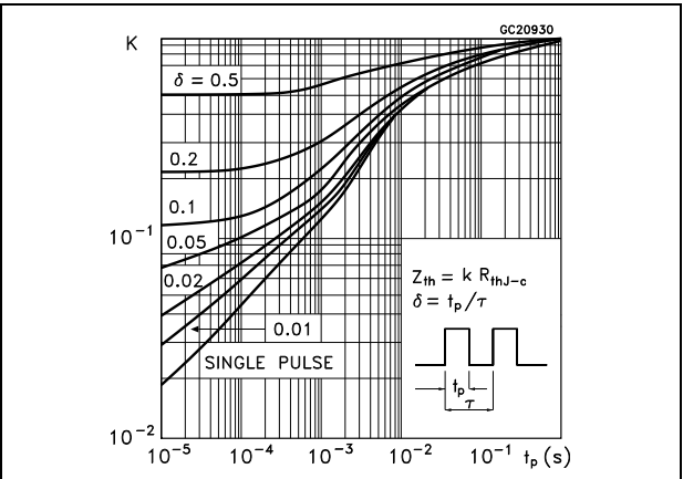
Figure 3. Thermal impedance
