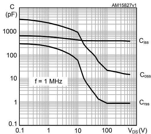
Figure 9. Capacitance variations
