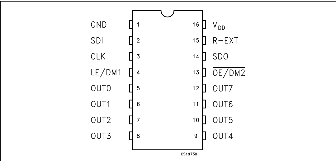
Figure 1. Pin connections
