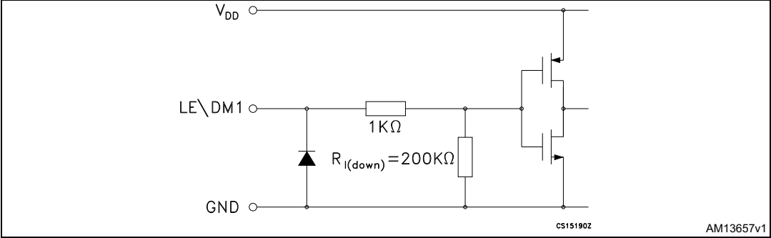
Figure 4. LE/DM1 terminal
