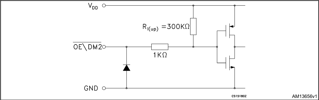
Figure 3. OE/DM2 terminal
