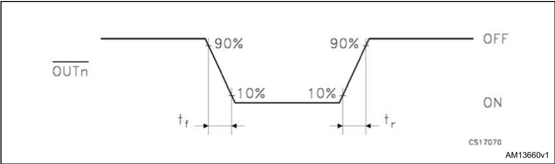
Figure 10. Outputs
