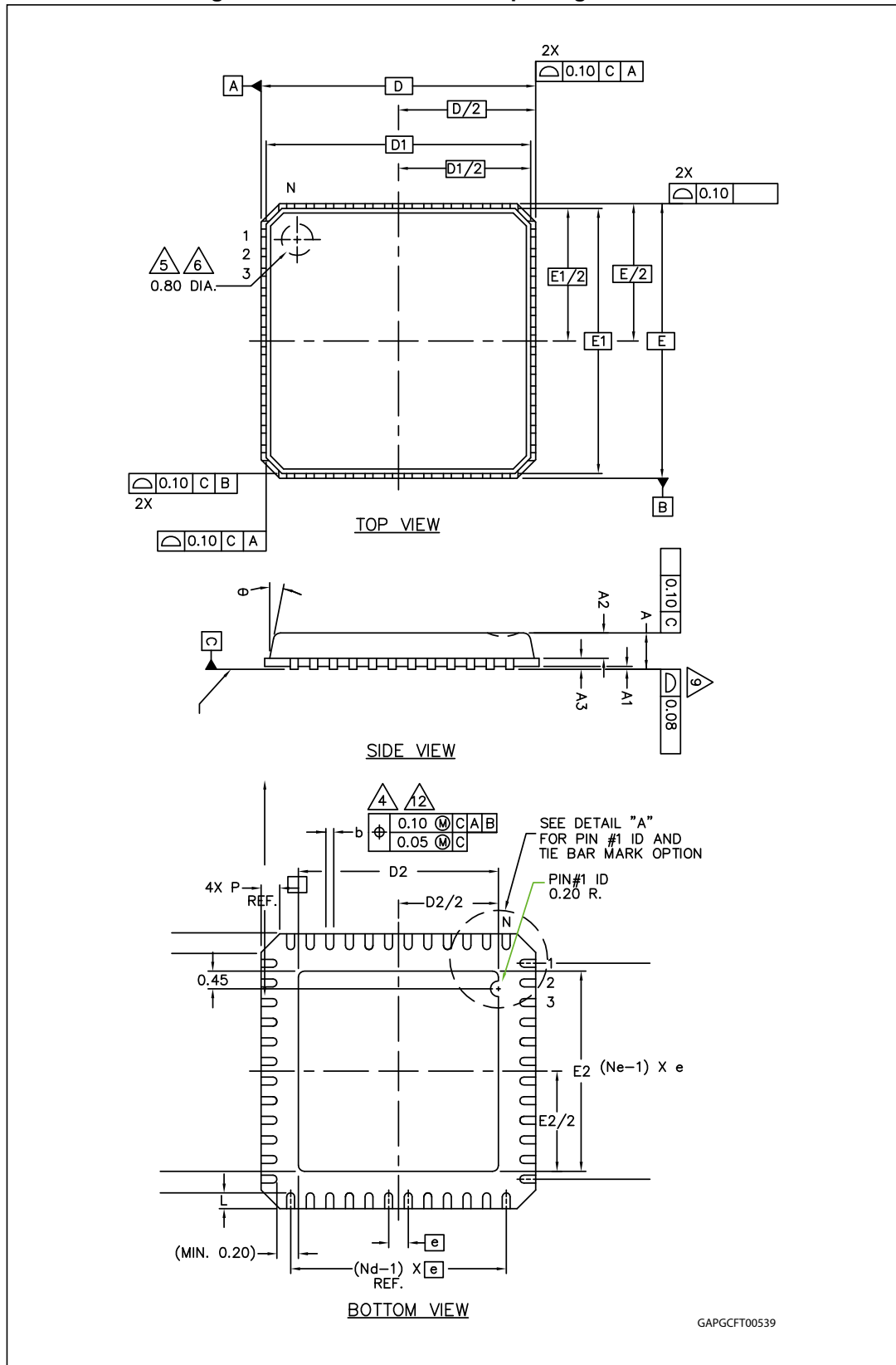
Figure 5. VFQFPN56 7 x 7 mm package dimension
