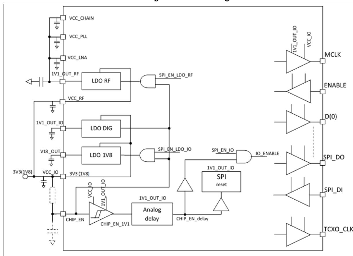
Figure 3. Power configuration
