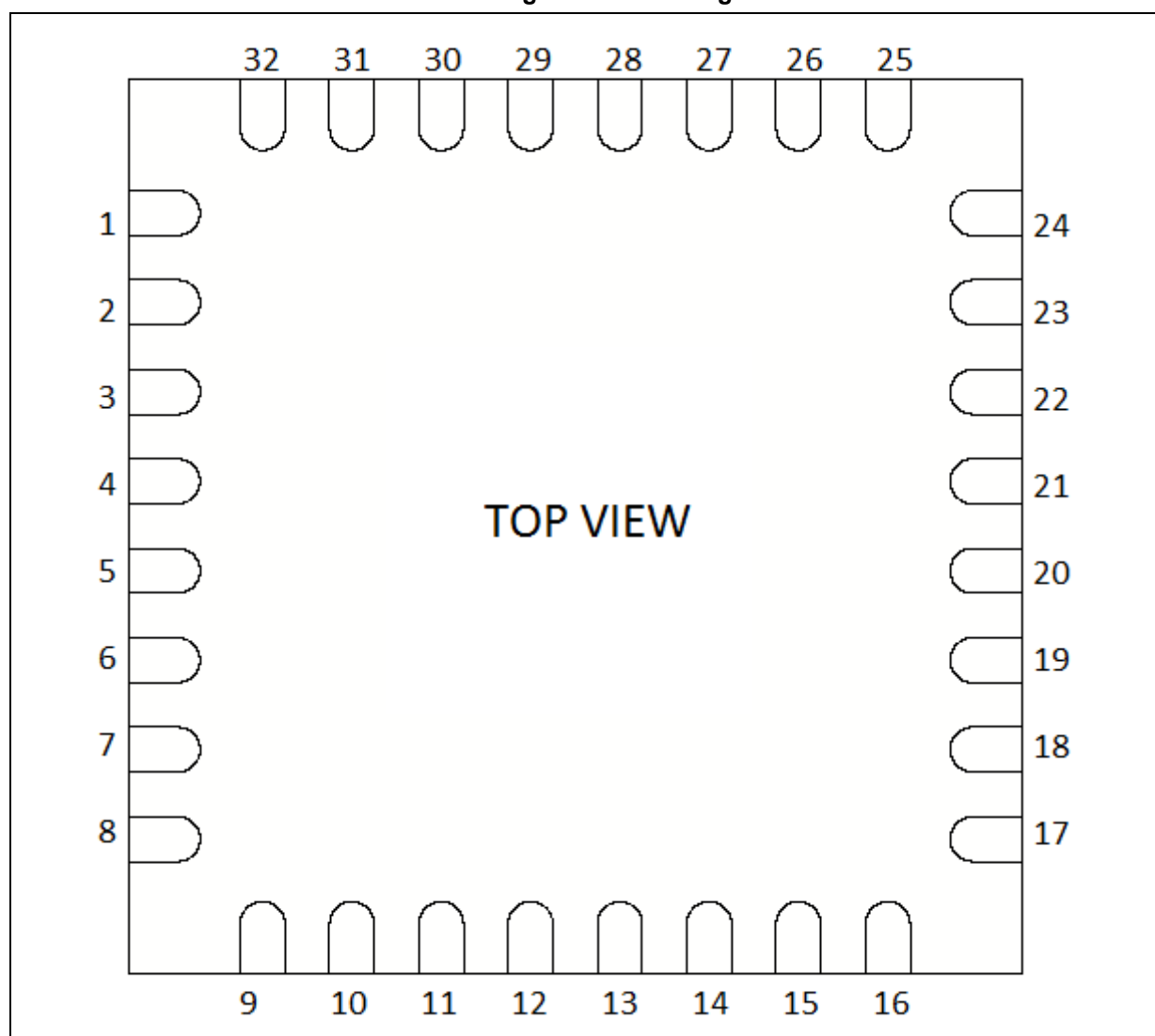
Figure 2. Pin configuration
