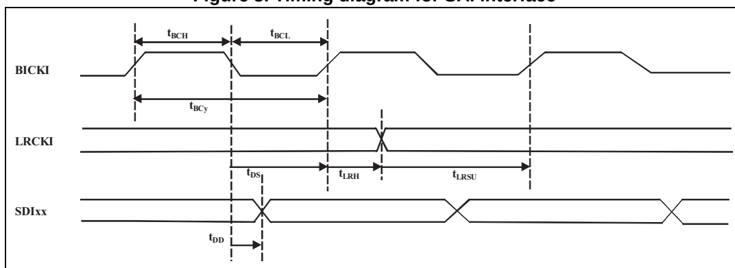
Figure 3. Timing diagram for SAI interface
