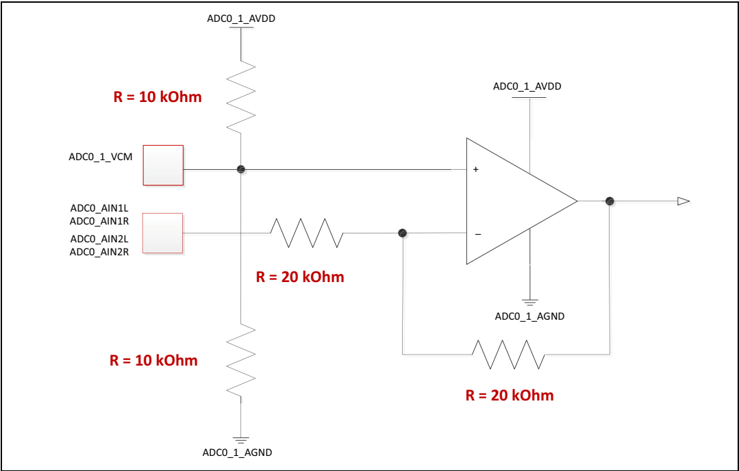
Figure 7. Audio ADC Input Equivalent Circuit
