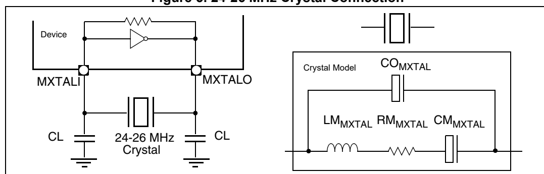
Figure 5. 24-26 MHz Crystal Connection
