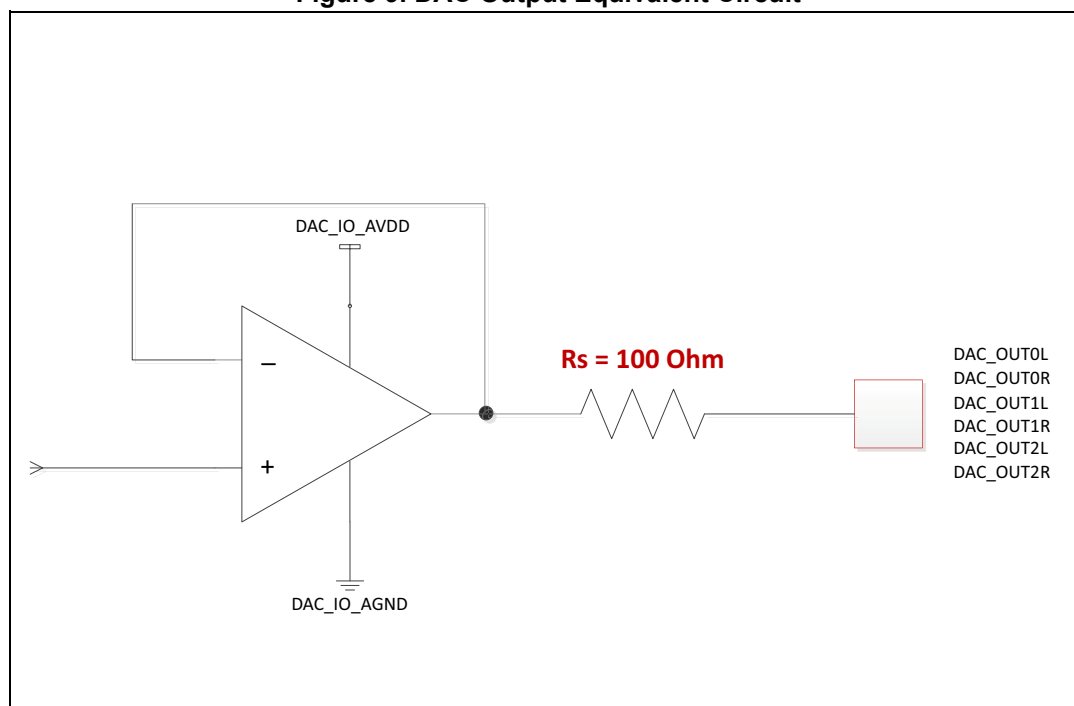
Figure 9. DAC Output Equivalent Circuit
