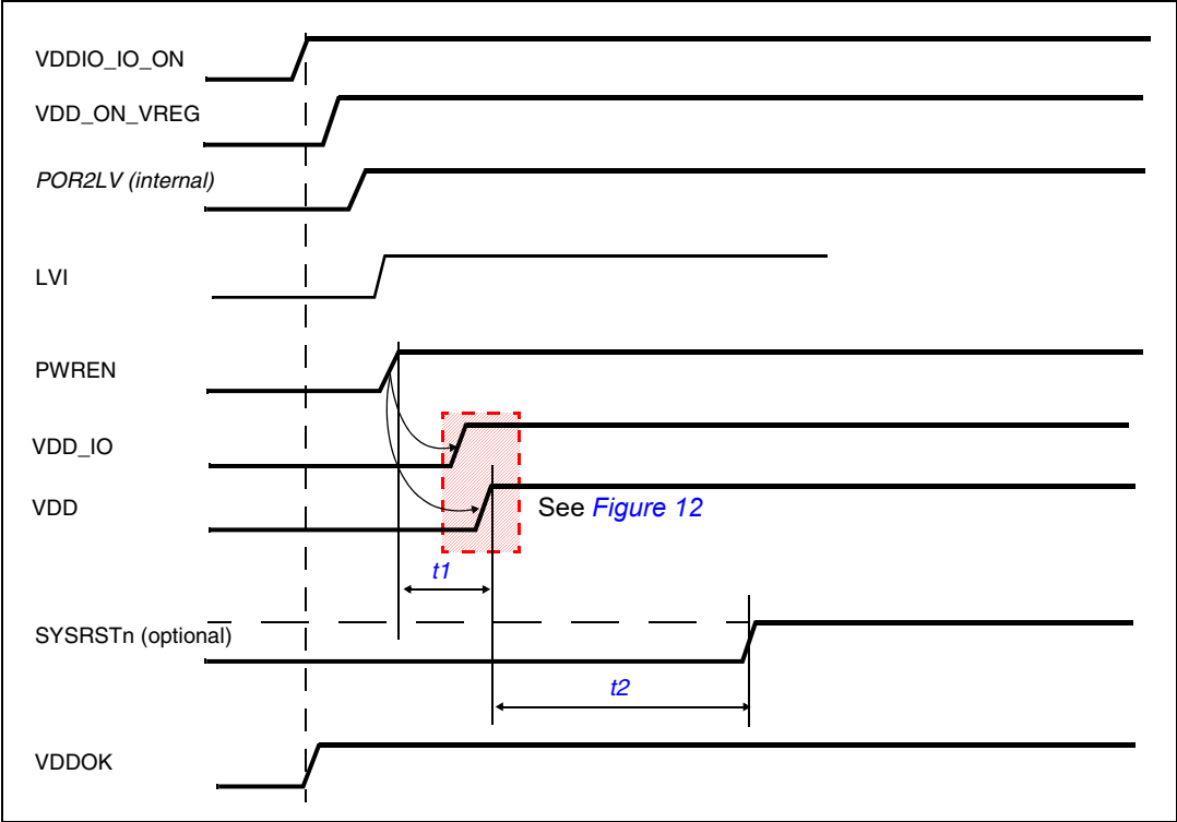
Figure 14. Initial Power-up Sequence (without VDDOK)
