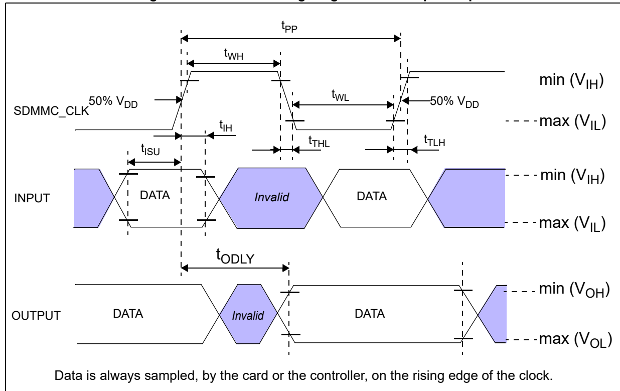
Figure 17. SD/MMC Timing Diagrams: Data input/output
