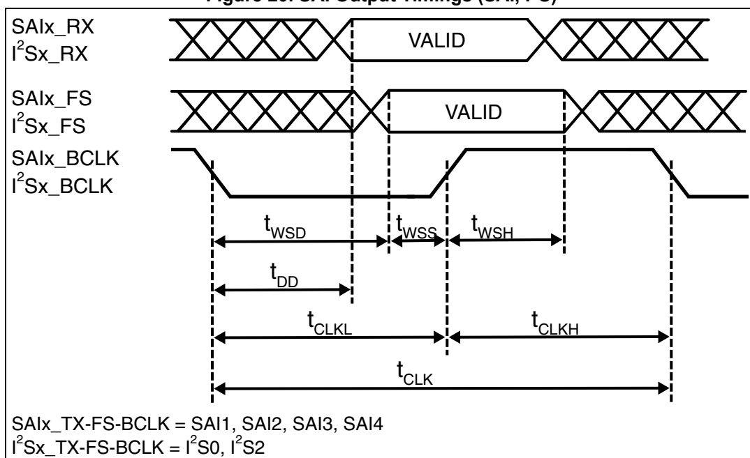
Figure 20. SAI Output Timings (SAI, I 2 S)
