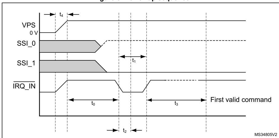
Figure 5. Power-up sequence
