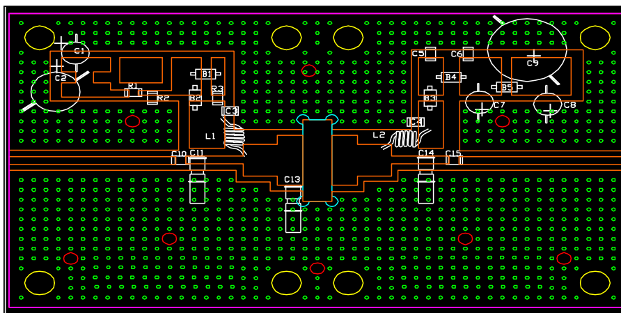
Figure 7. Circuit layout
