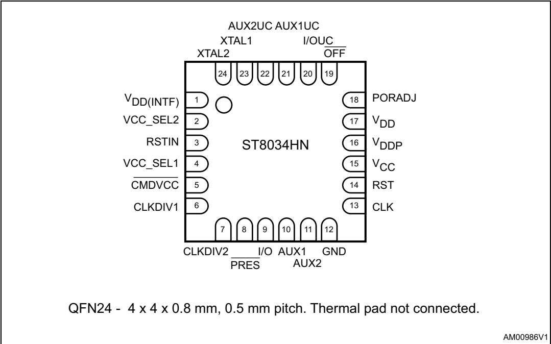
Figure 3. Pin connections ST8034HN (top-through view)
