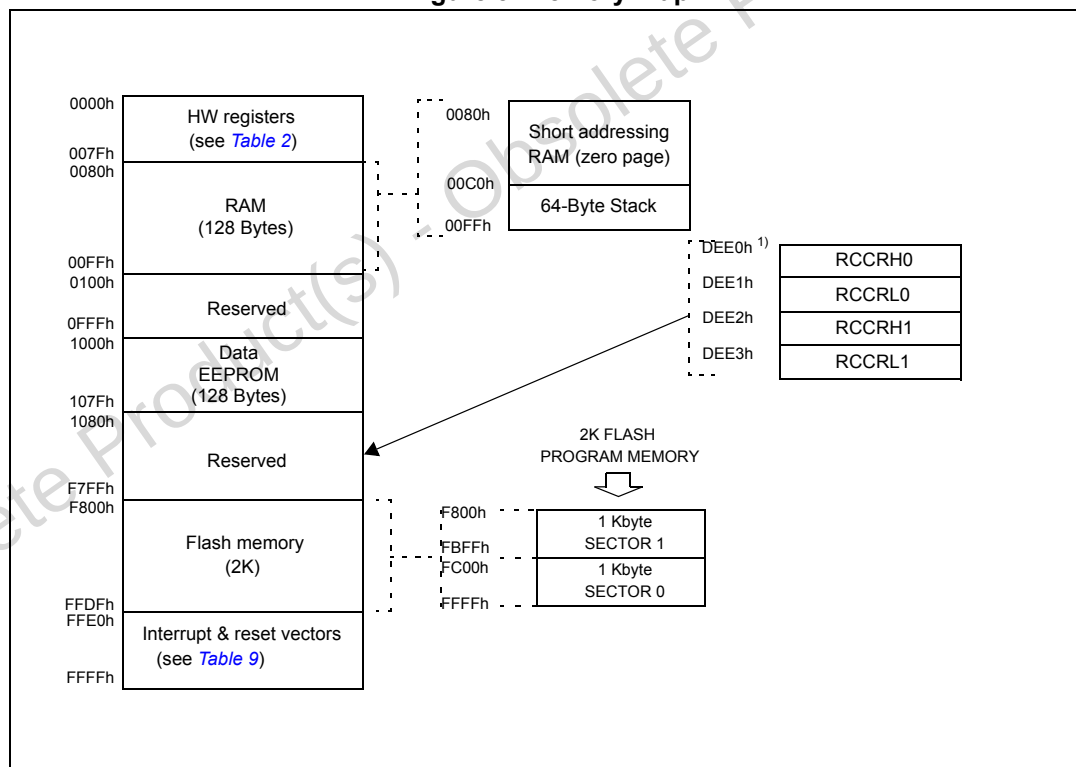
Figure 5. Memory map
