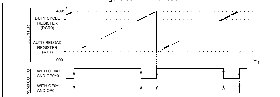
Figure 38. PWM function
