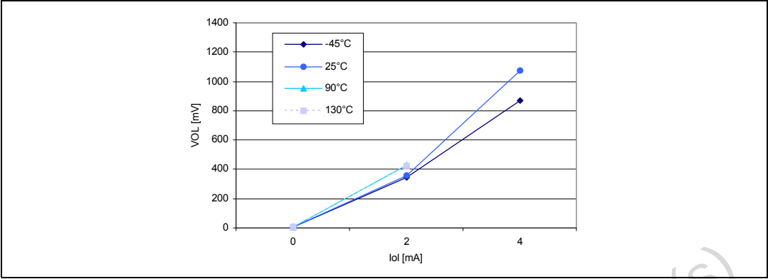
Figure 55. Typical V_{OL} at v_{DD} = 2.4\text{ V} (standard pins)
