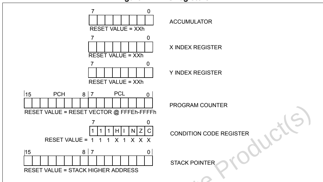
Figure 11. CPU registers
