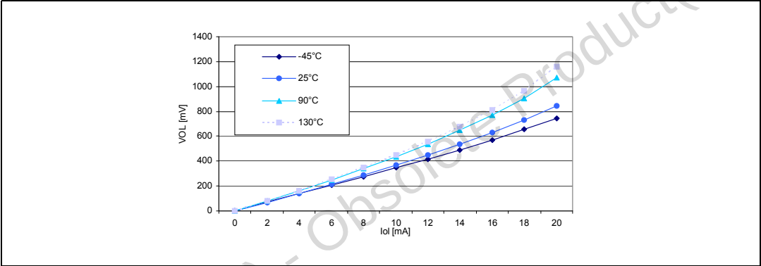
Figure 59. Typical V_{OL} at V_{DD} = 3\text{ V} (HS pins)
