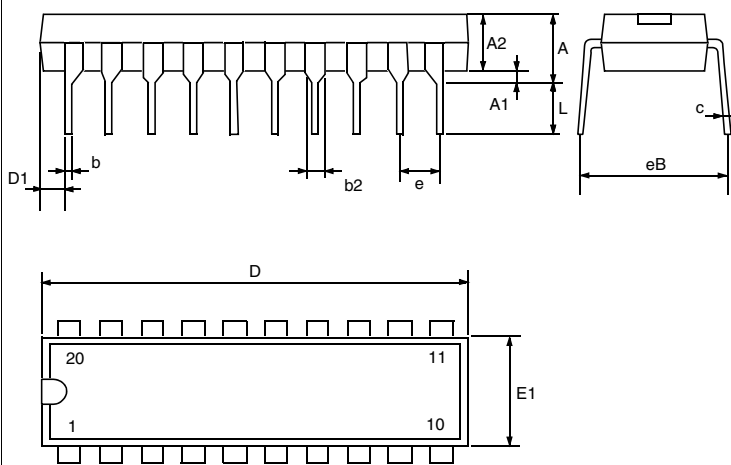
Figure 91. 20-Pin Plastic Dual In-Line Package, 300-mil Width
