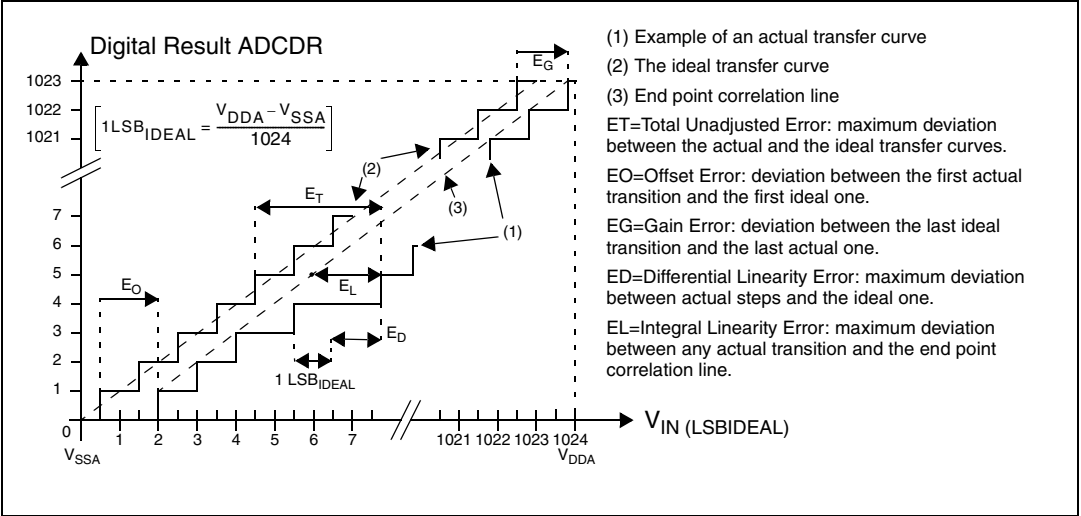
Figure 146. ADC accuracy
