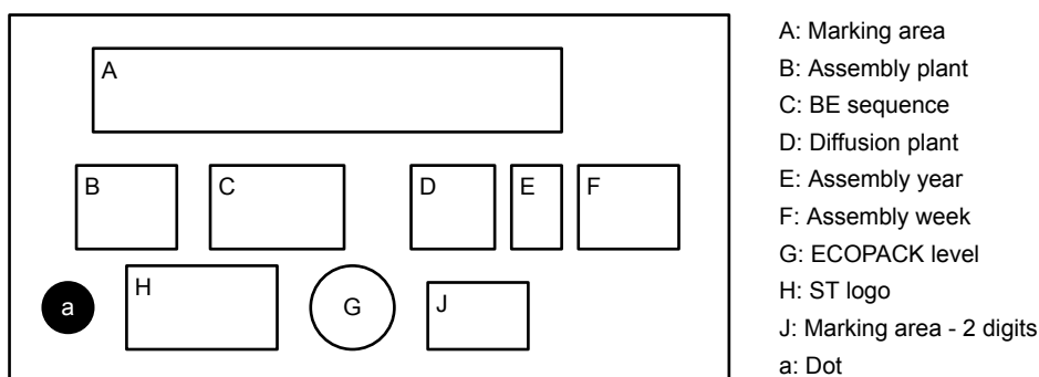
Figure 14. TSSOP28 device package marking area
