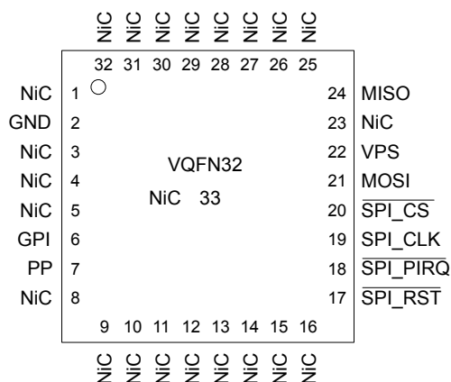
Figure 2. VQFN32 pinout
