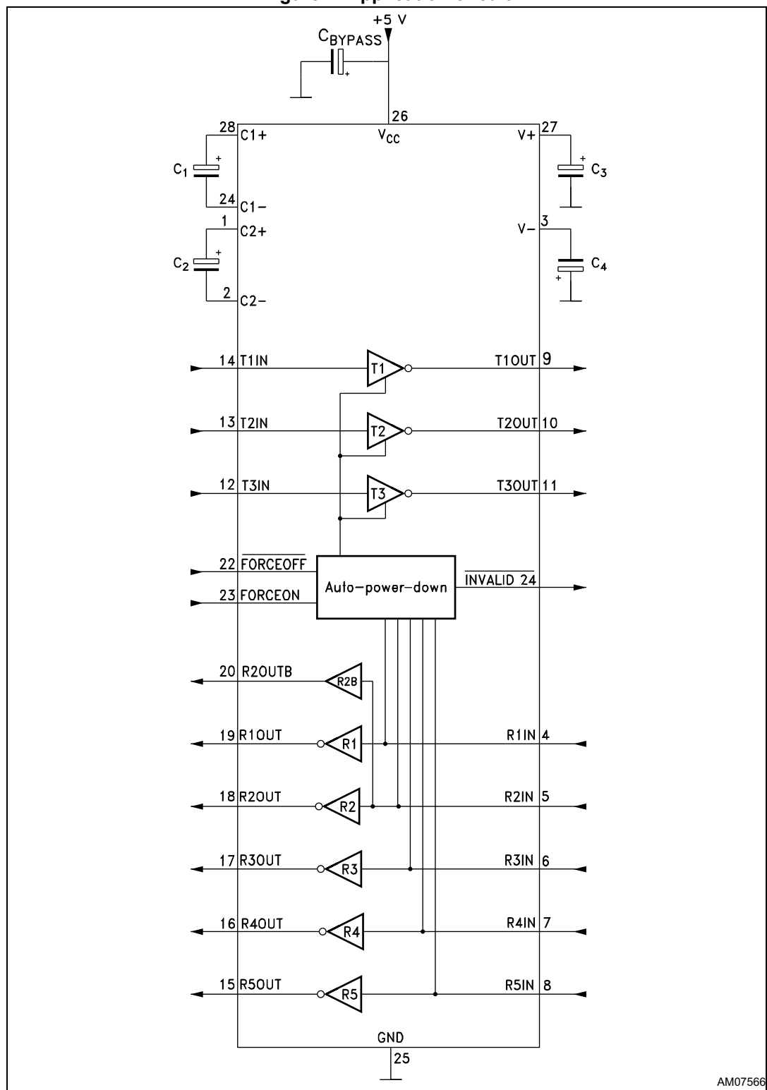
Figure 2. Application circuit
