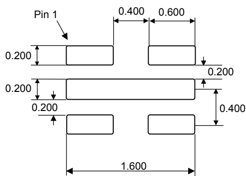
Figure 16. UDFPN5 - Recommended footprint
