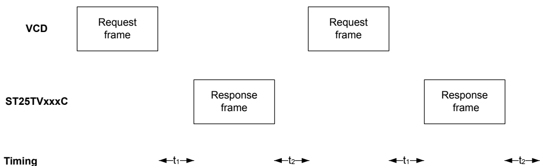
Figure 8. ISO15693 protocol timing
