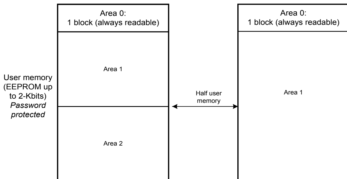
Figure 5. Memory organization
