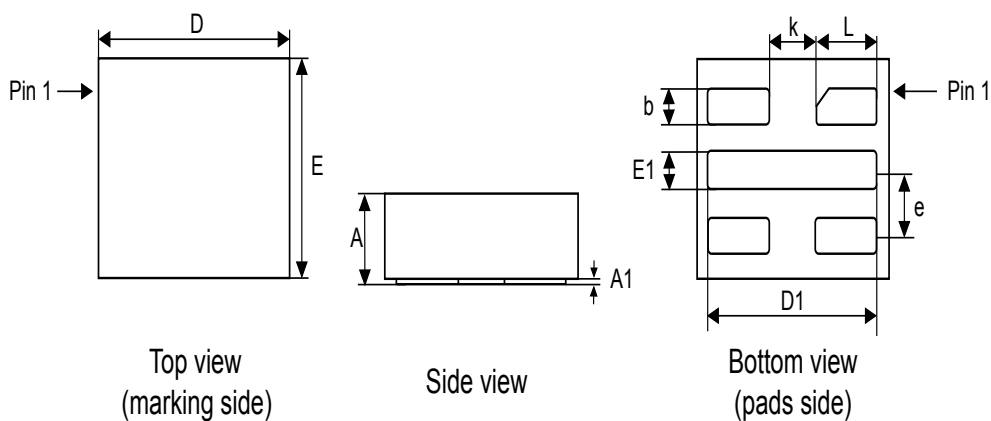
Figure 24. UFDFPN5 - 5-lead, 1.7 × 1.4 mm, 0.55 mm thickness package outline
