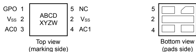
Figure 4. 5-pin package connections - ST25TA02KB-D
