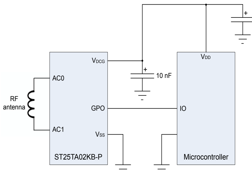
Figure 7. Applicative example of GPO usage - ST25TA02KB-P
