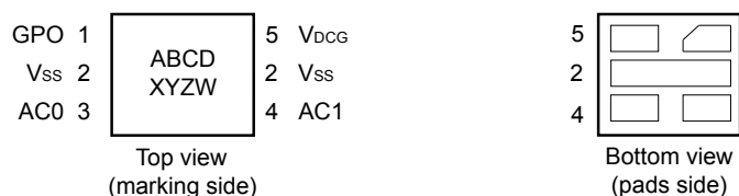
Figure 5. 5-pin package connections - ST25TA02KB-P
