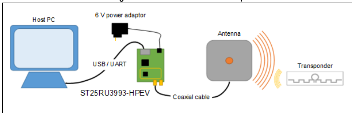
Figure 1. Standard connection setup
