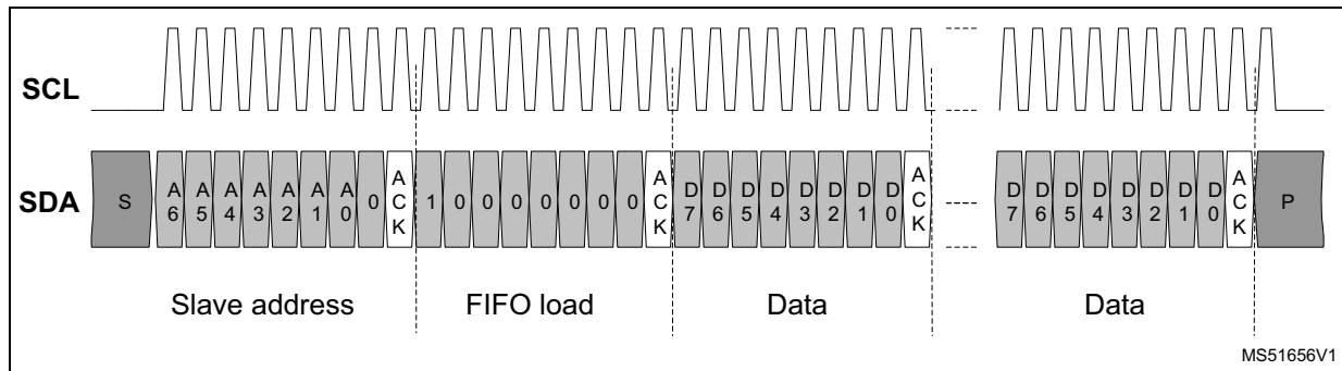
Figure 25. FIFO load
