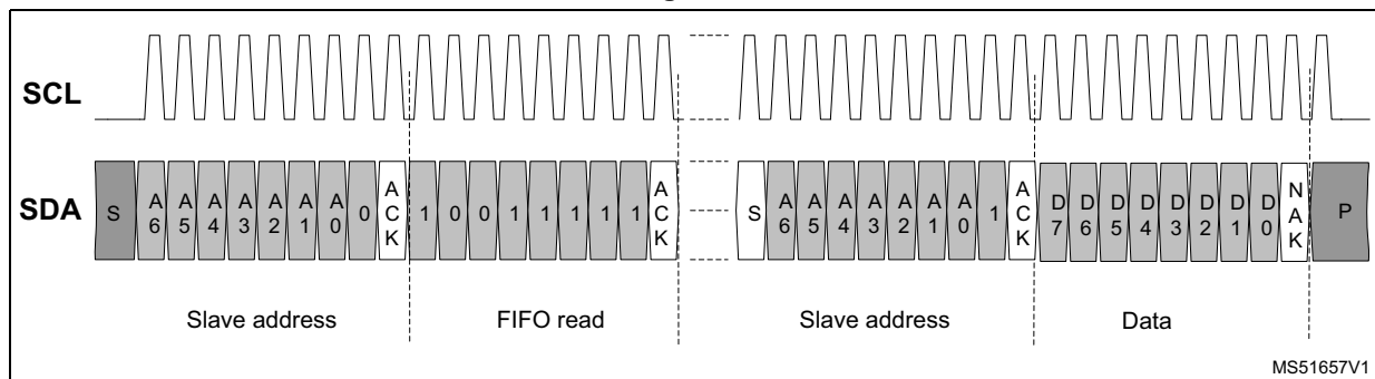
Figure 26. FIFO read
