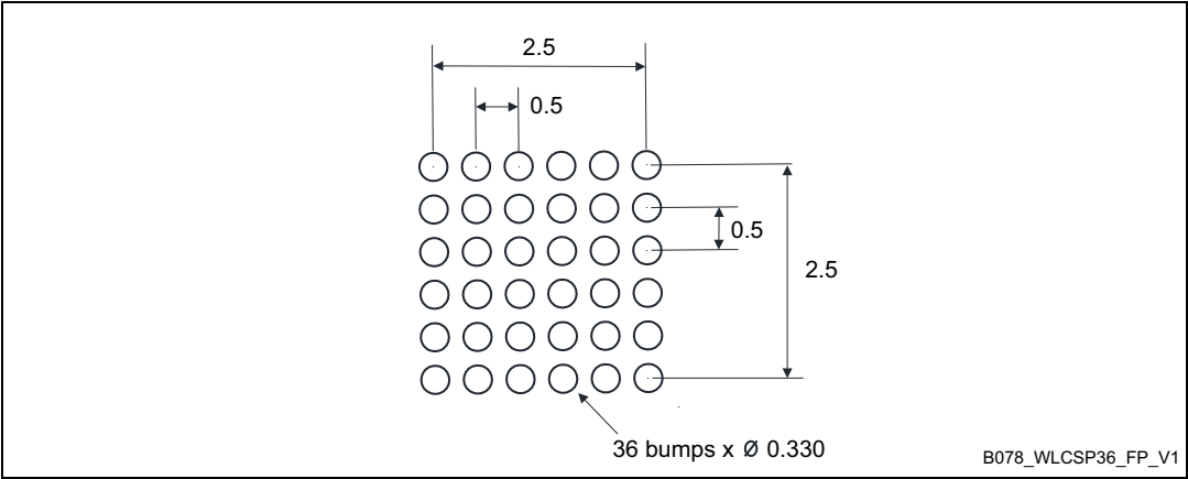
Figure 41. WLCSP36 - Footprint example
