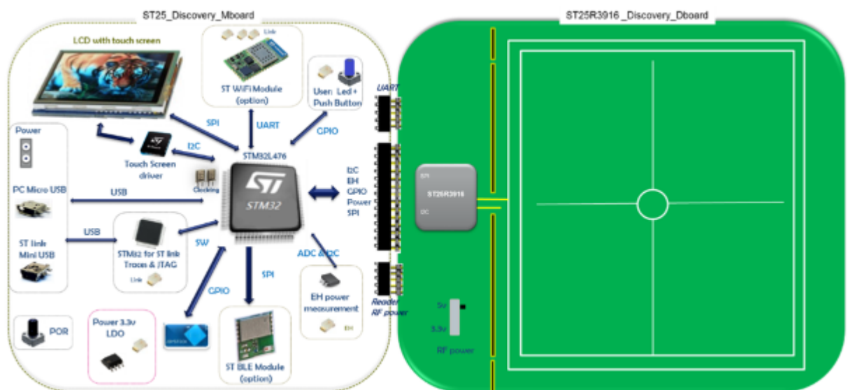
Figure 1. Connection scheme and diagram
