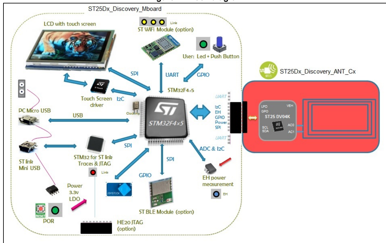
Figure 2. Block diagram
