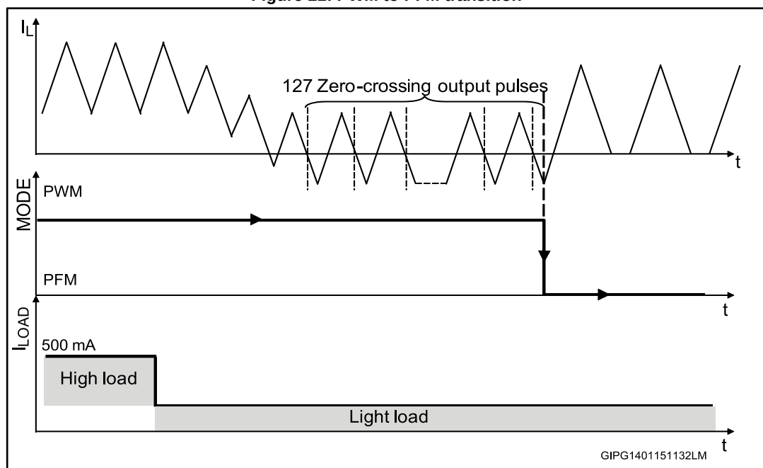
Figure 21: PWM to PFM transition
