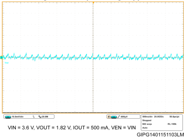
Figure 13: Output voltage ripple
