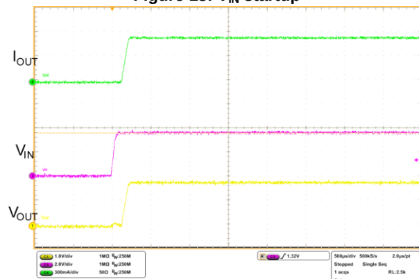
Figure 18: V_{IN} startup
